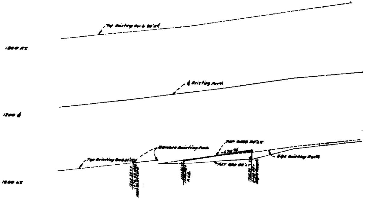
PROFILE CALIFORNIA STREET SCALE HORIZ: 1" = 40' VERT: 1" = 4'
