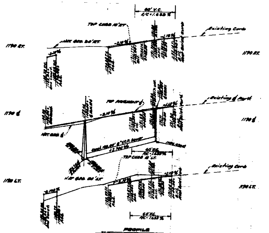
PROFILE FLORES STREET SCALE HORIZ: 1" = 40' VERT: 1" = 4'
